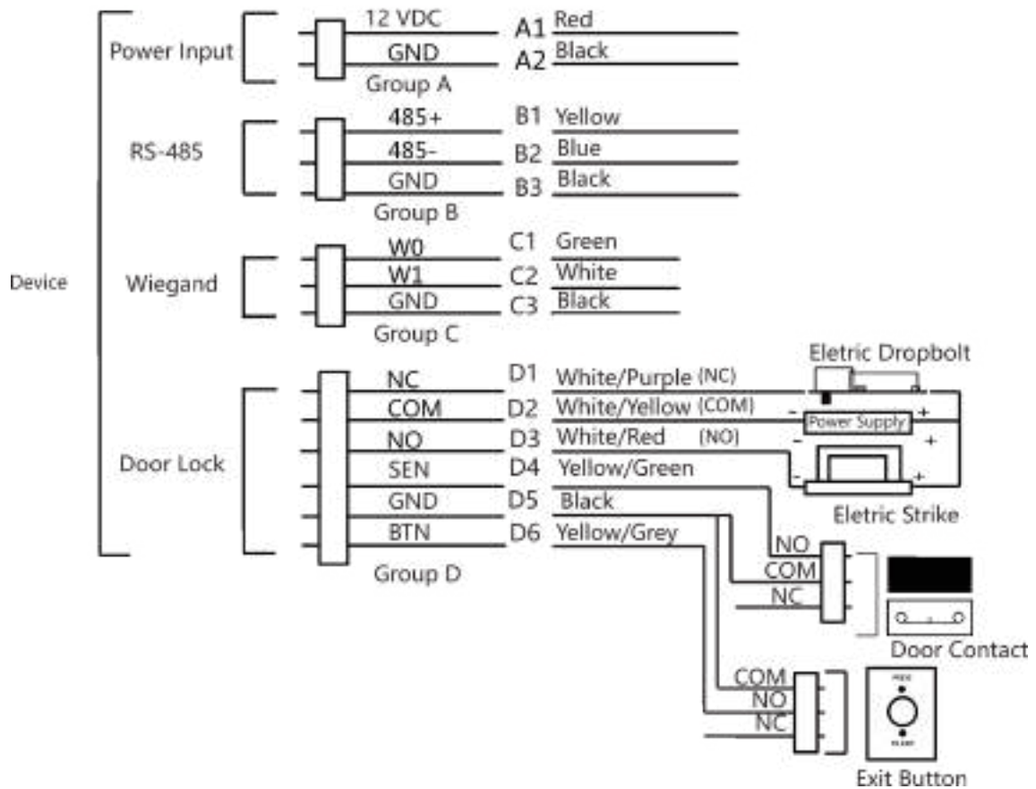
Figure 4-1 Device Wiring
