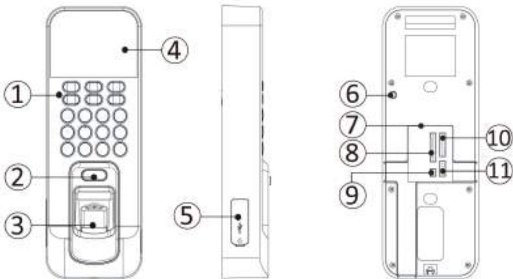
Figure 3-1 Device Appearance
