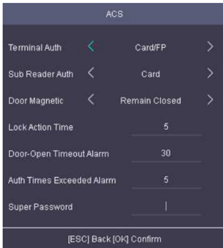
Figure 7-6 Access Control Parameters
