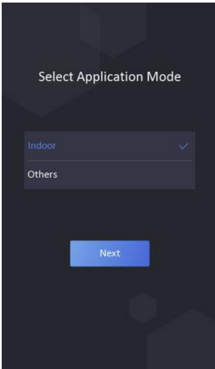
Figure 6-2 Welcome Page
