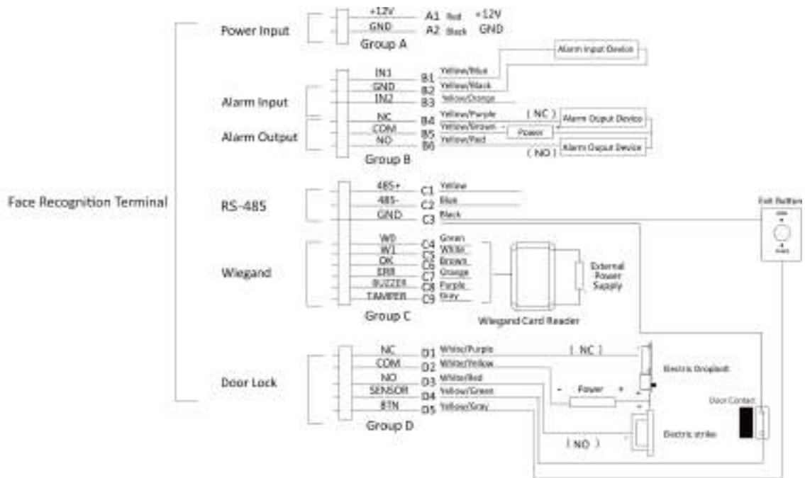
Figure 4-2 Device Wiring
