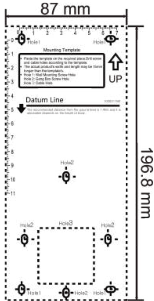
Figure 3-4 Mounting Template
