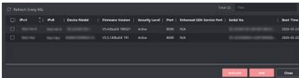
Figure 9-2 Online Device
