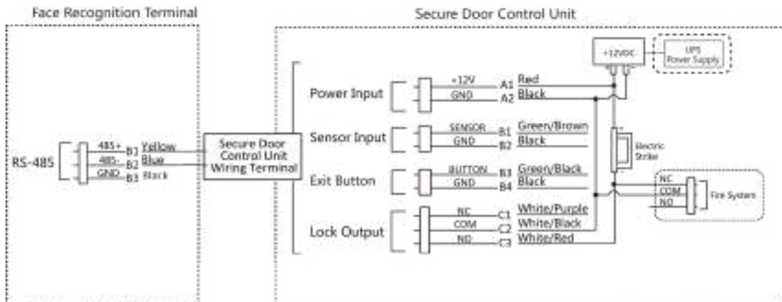
Figure 4-9 Wiring Diagram
